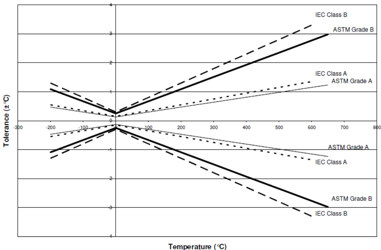
Figure 1.1 Standard PRT Interchangeability
