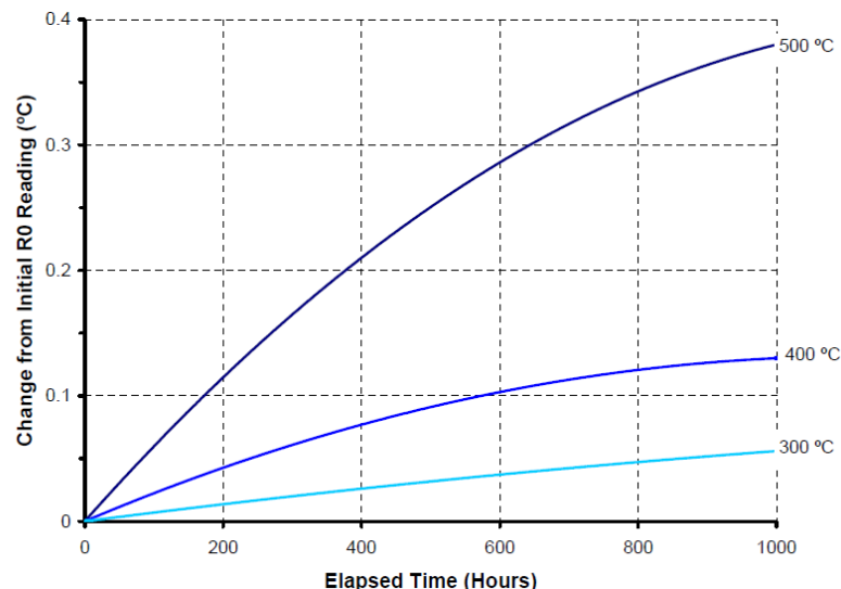
Figure 1. Typical change in ice point reading versus time at temperature, for an industrial grade RTD
