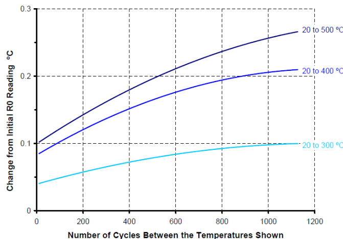
Figure 2. Typical change in ice point reading versus number of cycles between temperatures
